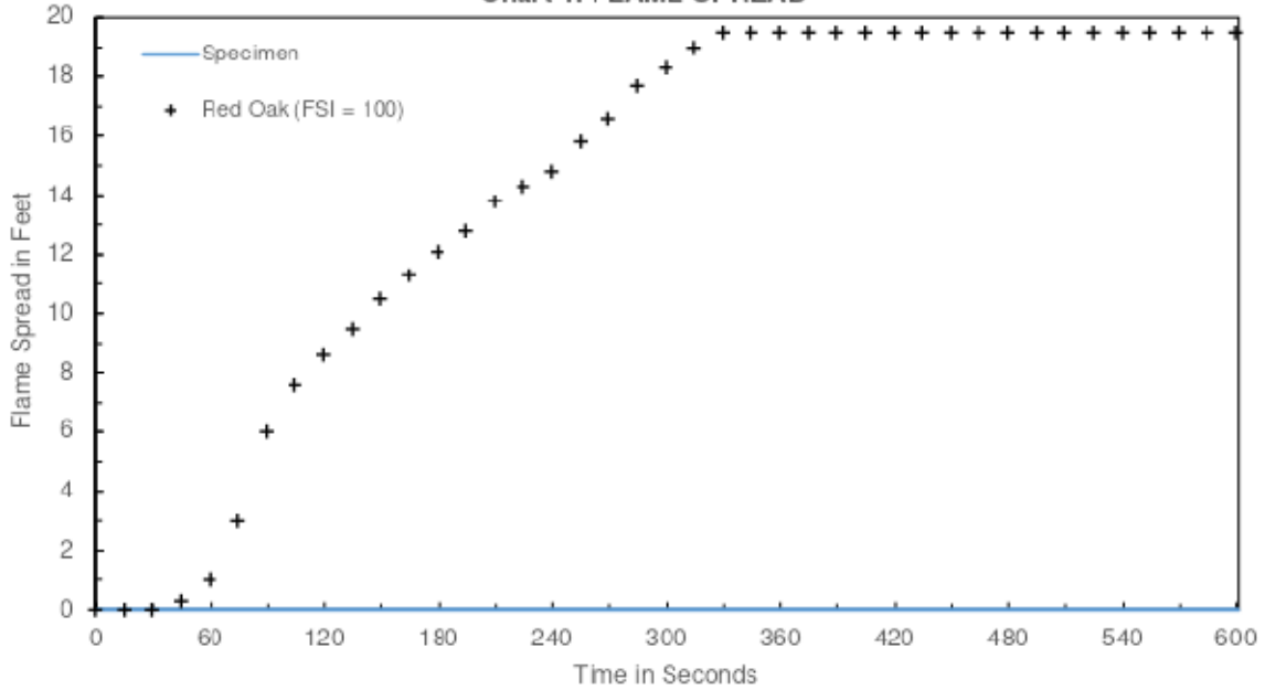
Chart 1. FLAME SPREAD
