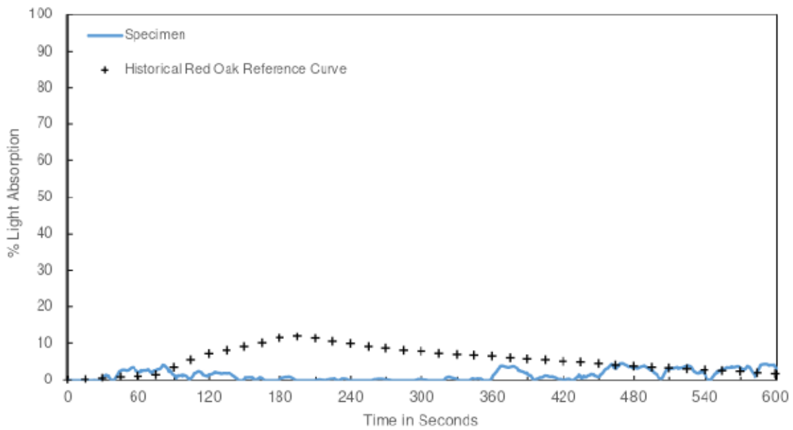
Chart 2. SMOKE DEVELOPED
